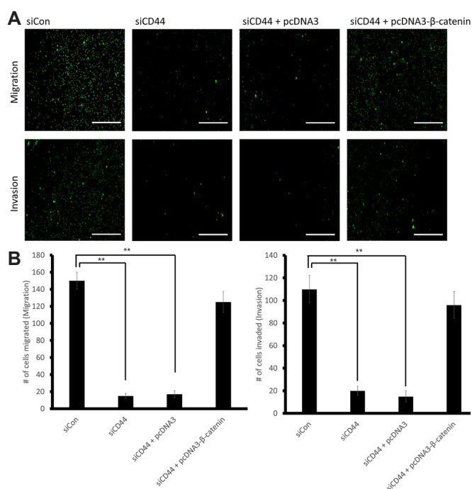
Figure 3. Migration and invasion assay on siRNA transfected (siCon a:d siCD44) and co-transfected (siCD44 + pcDNA3 and siCD44 + pcDNA3- \beta -catenin) MKN45 cells. (A) Representative images of migrated and invaded cells on the bottom of transwell inserts from siRNA transfected cells (siCon and siCD44), siRNA and empty vector co-transfected cells (siCD44 + pcDNA3), siRNA and \beta -catenin overexpressing vector co-transfected cells (siCD44 + pcDNA3- \beta -catenin). After 72 hour transfection, the cells were stained with CFDA to produce green fluorescence. The image was taken with a fluorescence microscope (Nikon). Scale bar: 500 \mu m (B) Quantification of migrated or invaded MKN45 cells. The number of green fluorescence cells were counted by Image J. In this test, two technical replicates from the two biological replicates were measured for the same treatment. Mean \pm S.D. was plotted with statistical significance (two-way ANOVA and Tukey test): **, p \leq 0.01 .
