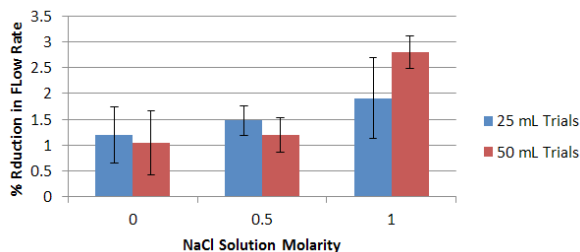
Figure 2: Change in flow rate due to introduction of a magnetic field. This figure shows the average reduction of flow due to the magnetic flow across 10 trials. The reduction value is the difference in flow rate of the magnetic and non-magnetic trials as a percentage of the non-magnet run. Error bars represent the standard deviation of 10 trials.
