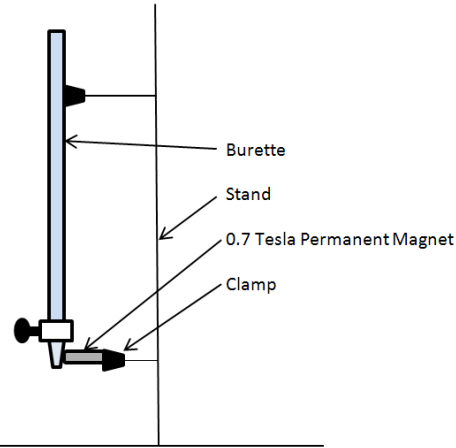
Figure 1: Experimental set-up. This figure shows a schematic depicting the position of the magnet in relation to the burette.
