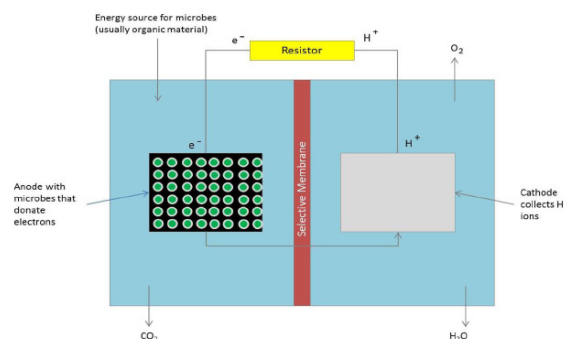
Figure 1: The mechanics of the microbial fuel cell.
