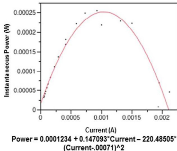
Figure 7: Power curve analysis. In a stabilized pMFC, resistance was modified in 30-second intervals and the corresponding voltage was recorded. Using said voltage data, power and current were both calculated, and power was plotted against current. Using previous research as justification, a quadratic regression was conducted, and a power curve (shown above) was generated (2). The regression had an r^2=0.93 with p<0.0001 , indicating a statistically significant quadratic relationship between instantaneous power and current; optimal resistance for maximum power output was determined to be 231 \Omega by optimizing the regression model.
