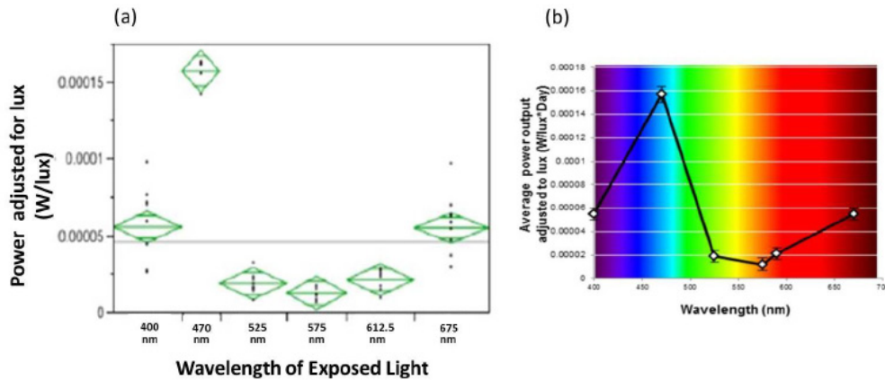
Figure 5: Analysis of differences in power over color. pMFCs were placed under various wavelengths of light using a color-changing LED, and voltage (and by extension power) was measured over a load of 10k \Omega . Lux was also measured using a lux meter and power was then normalized for lux. (a) shows average power outputs for each pMFC plotted per wavelength, with the green diamonds representing 95% confidence intervals. An ANOVA statistical test revealed statistically significant differences between the various wavelength groups ( p < 0.0001 ). (b) shows average power output variation plotted against the visible color spectrum. Note that the maximum power output was shown to be found at approximately 470 nm; while this does not correlate to the absorption spectra chlorophyll b or bacteriophyll, it does correlate to the spectra of some carotenoids found in R. rubrum (12,13).
