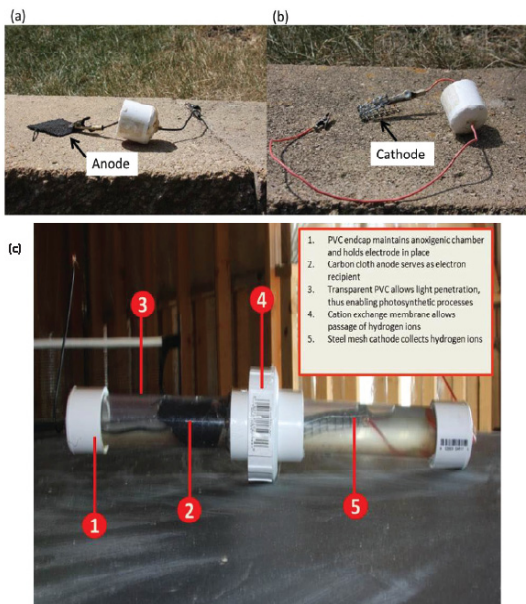
Figure 2: Potential pMFC prototype (constructed). Both electrodes were attached to PVC caps with epoxy and sealant in order to allow connection to main apparatus, which was also constructed from PVC piping. (a) The anode was constructed using a carbon cloth. It was connected to a circuit using an alligator clip. (b) The cathode was constructed using a folded stainless steel mesh. It was connected to the circuit using an alligator clip. (c) Depicted are the specifications of the final prototype pMFC developed.
