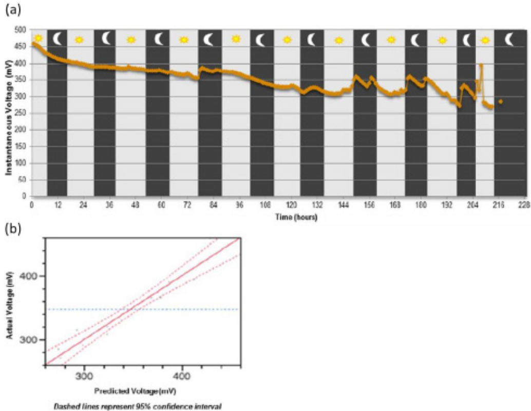
Figure 6: Analysis of pMFC exposed to natural sunlight conditions. A pMFC was kept in a greenhouse which allowed in natural sunlight, and both voltage over a 10 k \Omega resistor and lux (a measure of light intensity) were monitored over the course of several days. (a) depicts the raw voltage data as a function of time and additionally shows day and night periods. The voltage steadily but fairly slowly declined as a function of time, and some voltage peaks were seen in the night periods. (b) depicts a multiple regression analysis of voltage as a function of both time and lux. The results gave an r^2=0.94 with p<0.0001 and with 77% of variation accounted for in voltage attributed to time and the other 17% of variation accounted for in voltage attributed to lux. The predicted voltage was calculated using the multiple regression model and was plotted against the actual voltage. The dashed lines represent a 95% confidence interval, which when plotted against the actual v predicted line, demonstrates that the multiple regression model is highly accurate.
