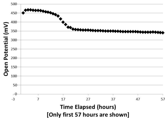
Figure 3: Proof of concept R. rubrum pMFC open potential over time. The prototype pMFC open voltage was measured over an extended period of time. The pMFC drops approximately 100 mV within the first 24 hours; note that hours 58 through 167 are not depicted due to the high consistency of the data.
